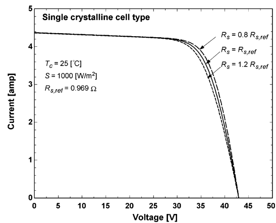
Fig. 2. Effect of series resistance for the single crystalline cell at standard rating conditions.
