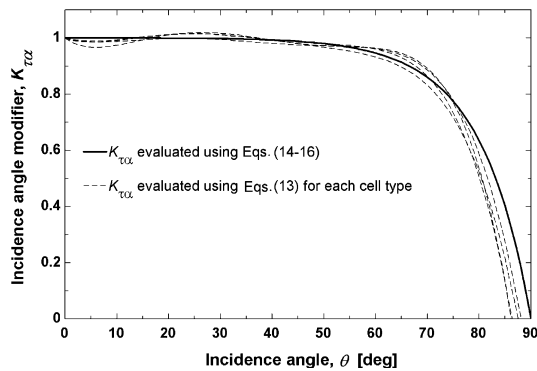
Fig. 4. Incidence angle modifier, K_{\tau z} , as a function of incidence angle, \theta , calculated using Eqs. (14)–(16) (solid line). The dotted lines are the incidence angle modifiers calculated using Eq. (13) with the coefficients for each cell type provided in Table A.1.
