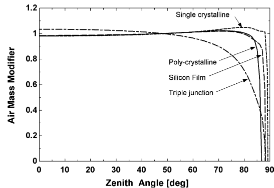
Fig. 5. Air mass modifier, M/M_{\text{ref}} , as a function of zenith angle, \theta_z , calculated using Eq. (17) with the coefficients for each cell type listed in Table A.1.
