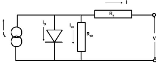
Fig. 1. Equivalent circuit representing the five-parameter model.
